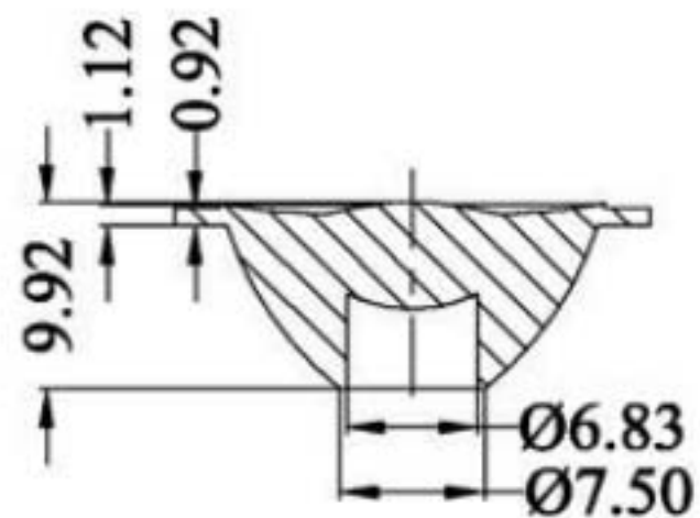
LENS
