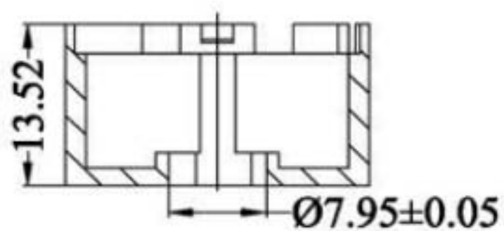
HOLDER
