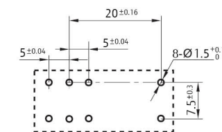
PIN PITCH 2 - FORM C
