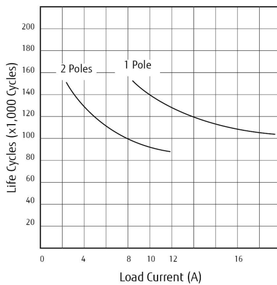
Electrical Endurance Curve NO: 277VAC Resistive 1s ON / 1s OFF
