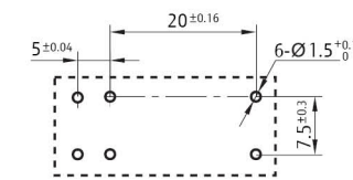
PIN PITCH 2 - FORM A
