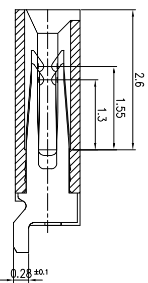
SEC A - A"
