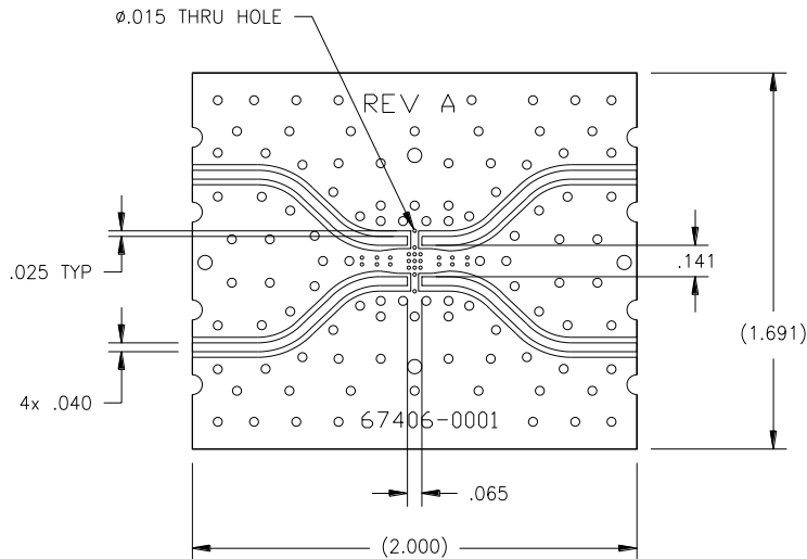
3 dB and 5dB Test Board
