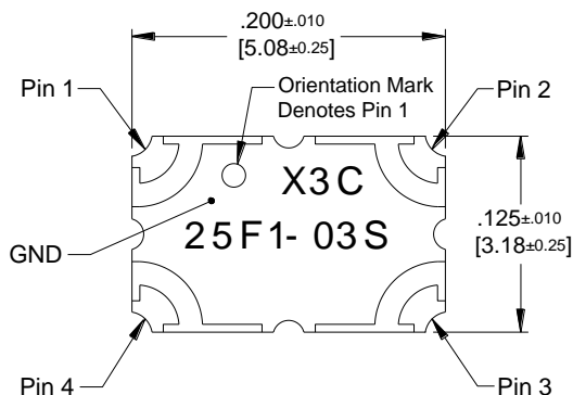
Dimensions are in Inches [Millimeters] X3C25F1-03S Mechanical Outline
